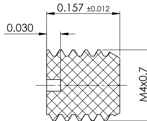
SECTION Y-Y
